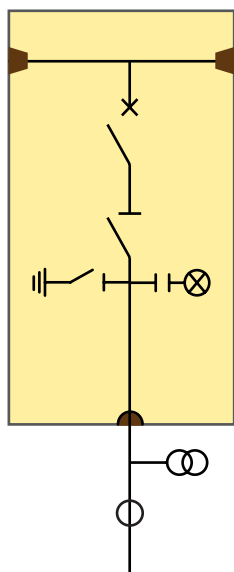
Single Line
